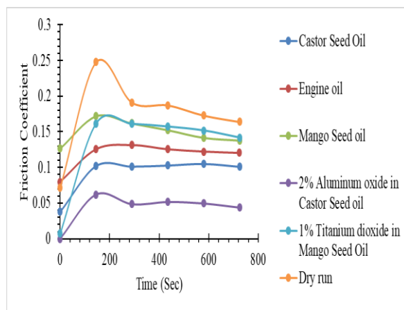
Figure 1: Friction Coefficient Against Time for Mango and Castor Seed Oils (Ameh, et al. , 2021)
