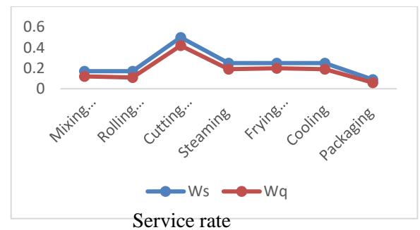
Figure 3: Meantime Spent in the Whole Process and Meantime Spent in the Queue
