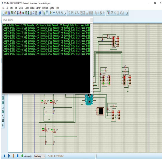
Fig 13. Lane Population Detection giving preference to Mummy B ignoring Tombia GRA lane
